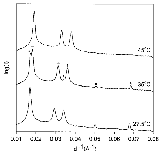
FIGURE 4 X-ray powder diffraction patterns obtained from MADGlcDAG with 20 wt% water. The acyl chain composition of MADGlcDAG is given in Table 1. At 35°C, the reflections arising from the gel phase are marked by a star and those from the H_{\text{II}} phase by a plus sign.
