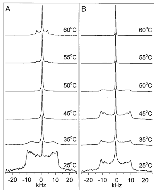
FIGURE 5 ^2H -NMR spectra of MGlcDAG with an acyl chain composition given in Table 1. (A) 10 wt% ^1H_2O . The fractions of the two phases at 55 and 60°C were obtained from simulations of the spectra and were estimated to be 32% H_{II} and 68% I_{II} at 55°C, and 58% H_{II} and 42% I_{II} at 60°C. (B) 20 wt% ^1H_2O . The fractions of the two phases at 45°C were estimated to be 85% L_{\alpha} and 15% I_{II} .
